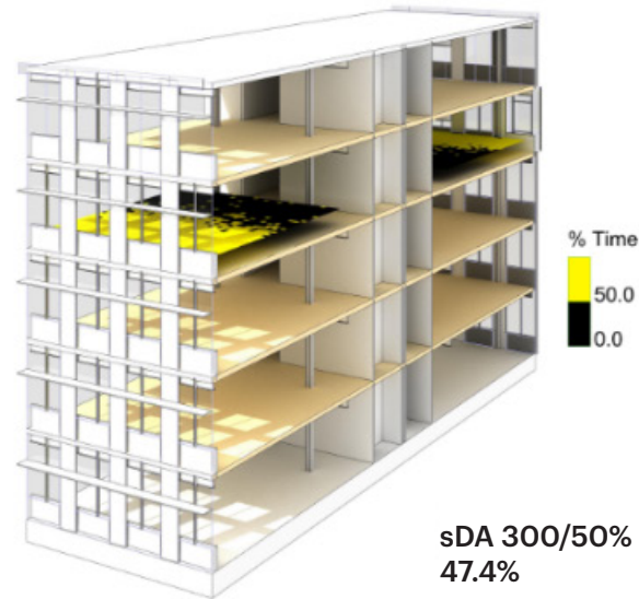
Baseline Steel/Concrete with External Overhang
