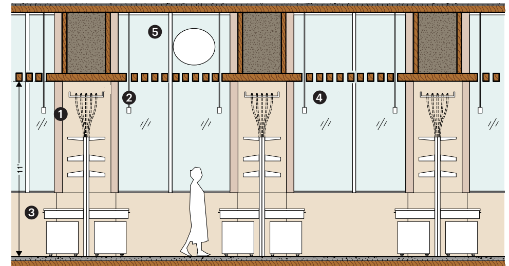
BSL 1 Open Lab Area - Wood Slats or Solid Ceiling Panels
