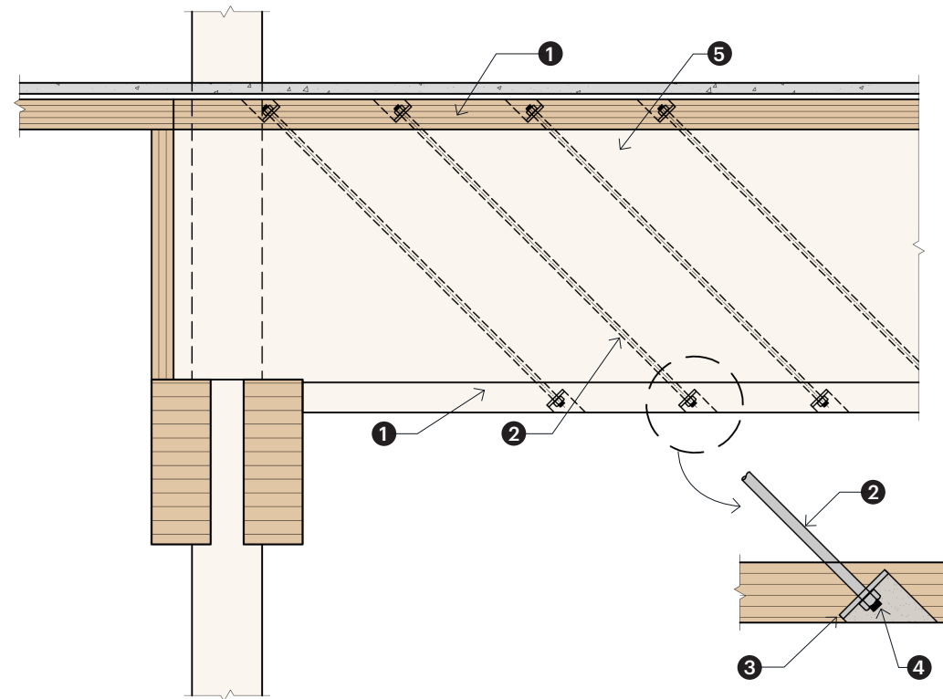
Elevation of floor beam
