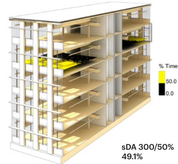
DES's Mass Timber with External Overhang
