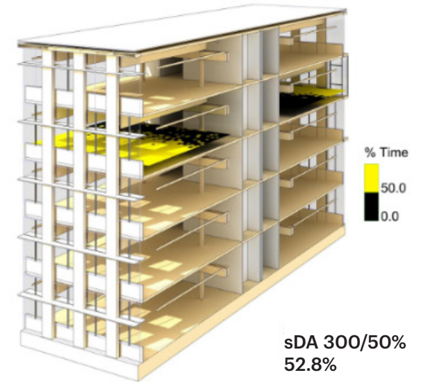
DES's Mass Timber with External Overhang and Internal Light Shelf
