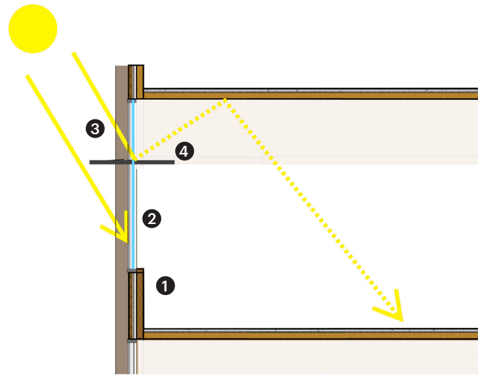
Light shelf concept (illustrative, summer solstice)
