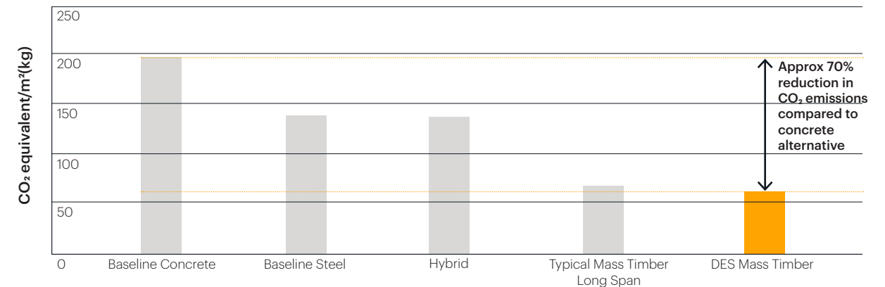
(A) CO 2 Emissions (A1-A3) from all Structural Alternatives
