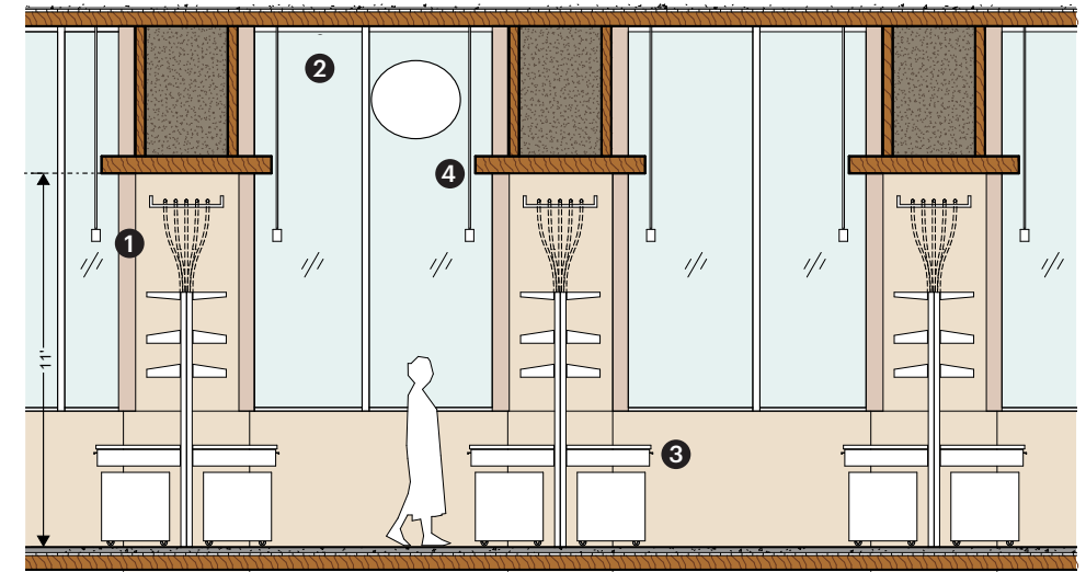
BSL 1 Open Lab Area - Exposed Wood Soffit
